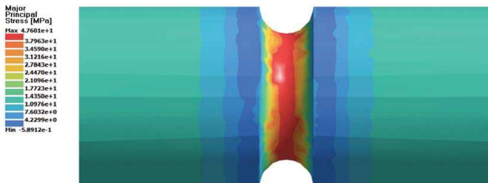
Figure 13: Maximum principal stress - SimSolid – Maximum accuracy – Benchmark 5
